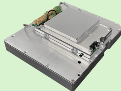
12.7×11.0×3.6cm/575g 10Watts×2/20Watts×2 (7Z030/7Z035) (Air to G. 150~300/250~500KM)
